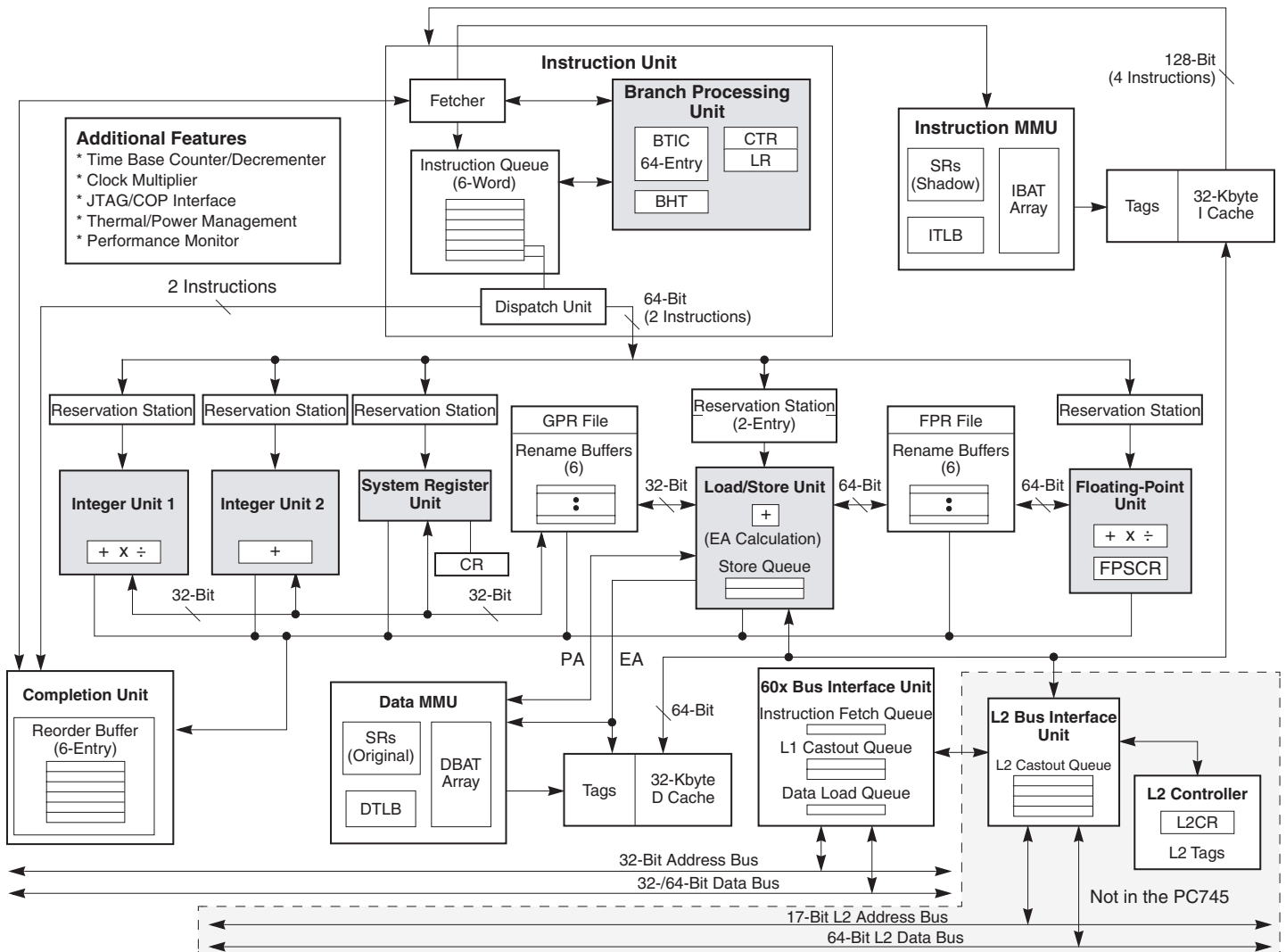
Figure 1-1. PC755 Block Diagram
