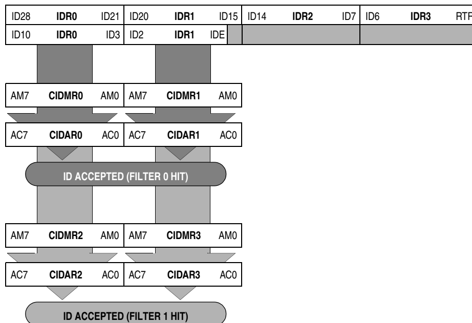
Figure 16-4. Dual 16-Bit Maskable Acceptance Filters
