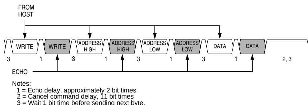
Figure 15-7. Write Transaction
