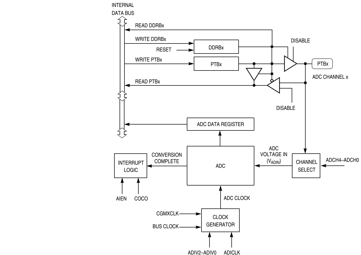
Figure 5-1. ADC Block Diagram
