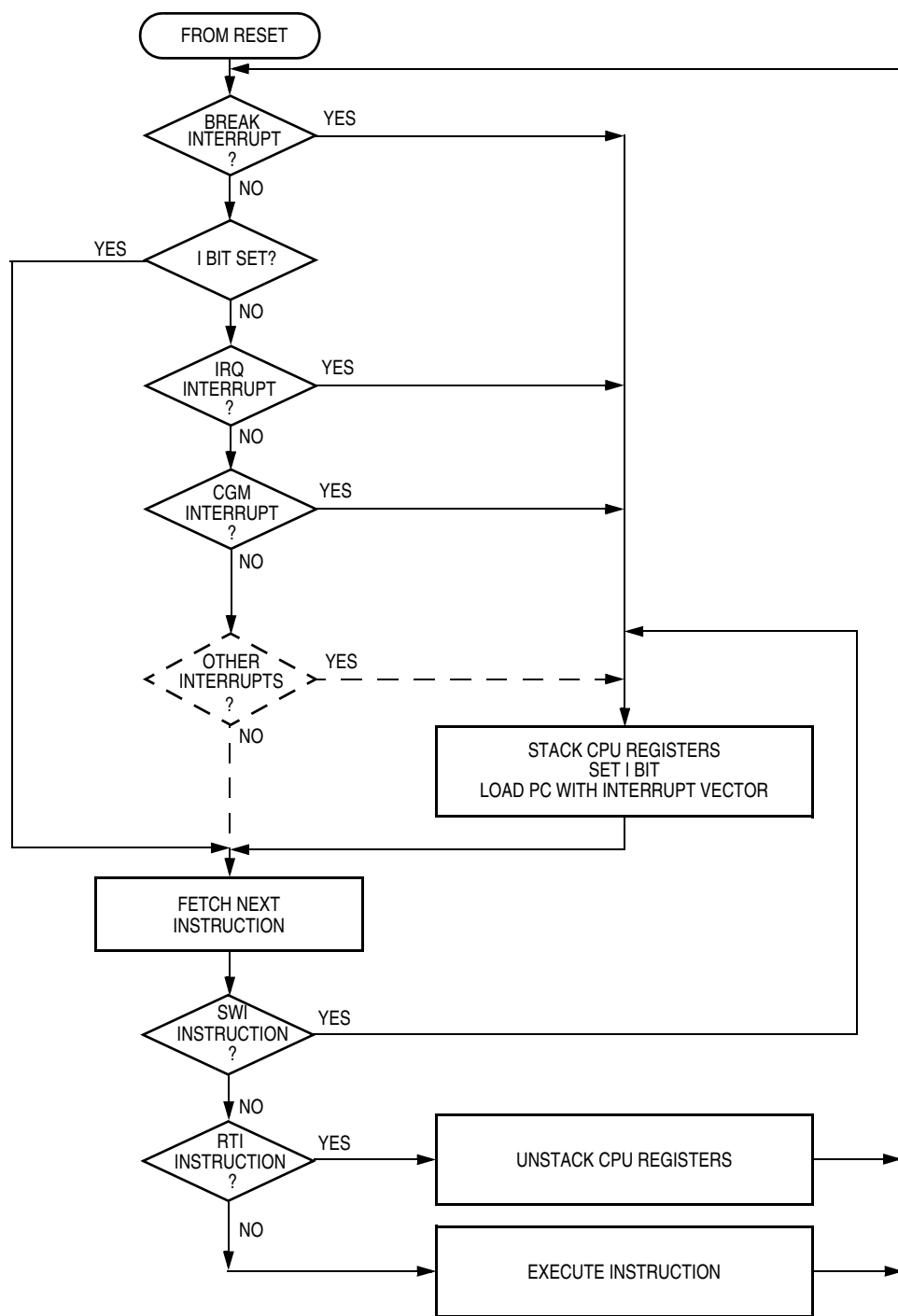
Figure 4-5. Interrupt Processing
