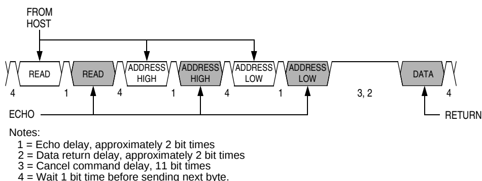
Figure 15-6. Read Transaction
