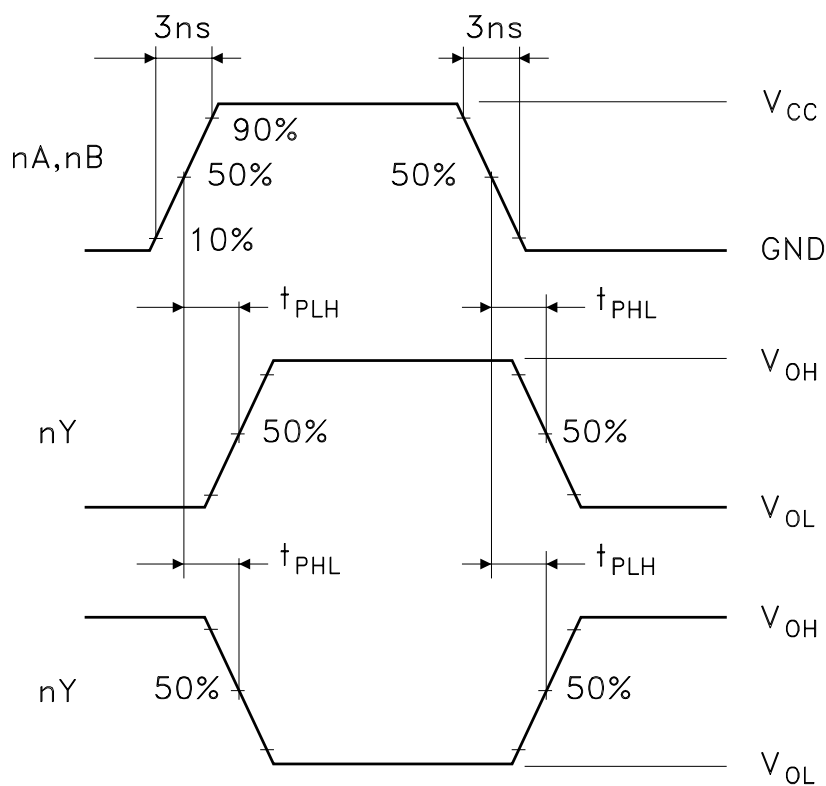
Figure 4: Waveform - Propagation Delays ( f=1\text{MHz} ; 50% duty cycle)
