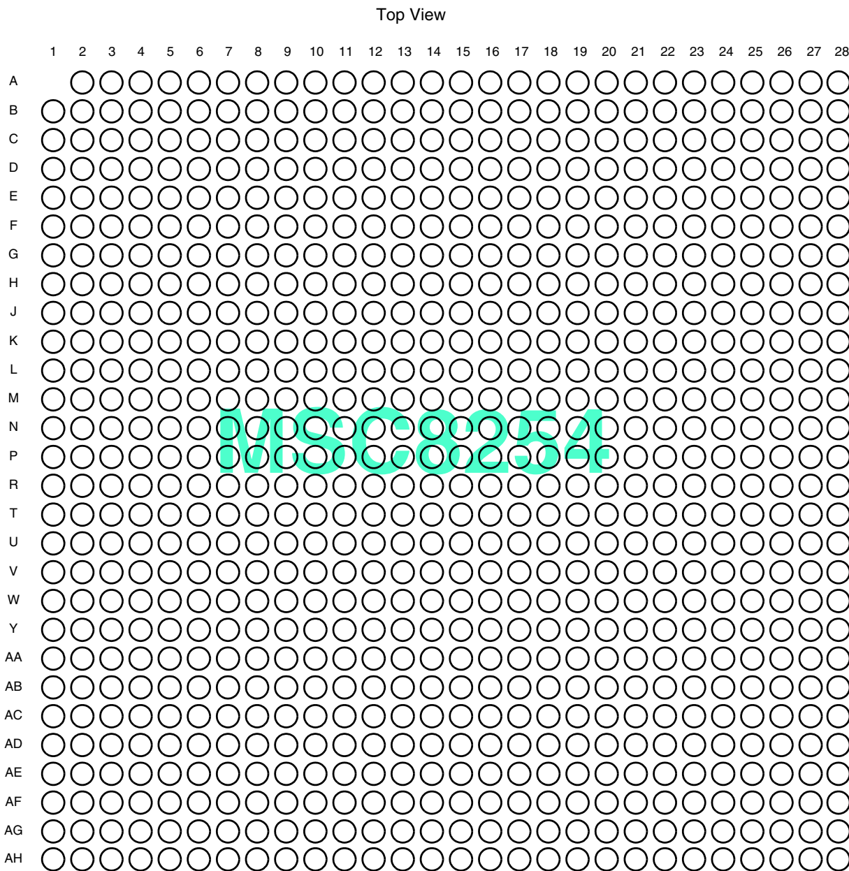
Figure 3. MSC8254 FC-PBGA Package, Top View
