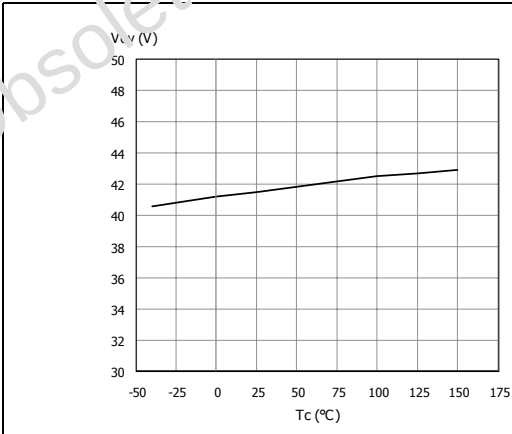
Figure 11. Over voltage shutdown
