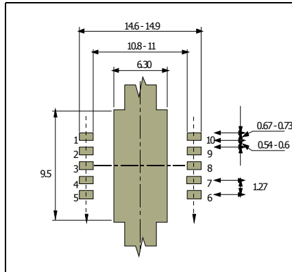
Figure 32. PowerSO-10 suggested pad layout
