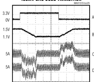
400mV DAC CODE TRANSITION
