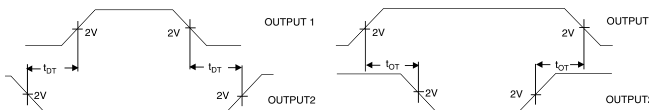
Figure 2. Deadtime and Overlap Time Measurements
