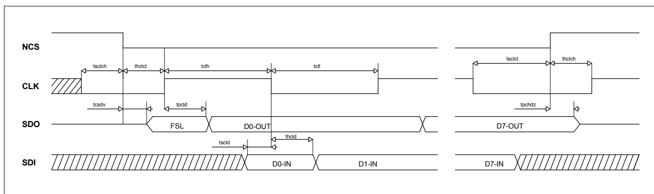
Figure 17 SPI Timings
