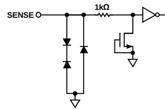
Figure 13. Equivalent SENSE Circuit
