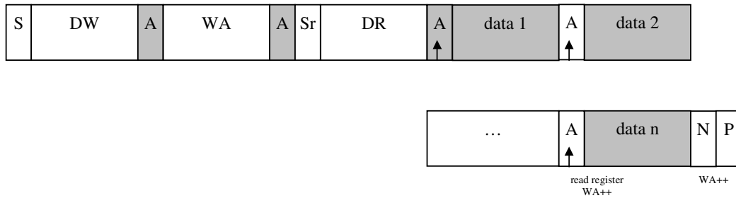
Figure 4 – I^2C Sequential-Read:
