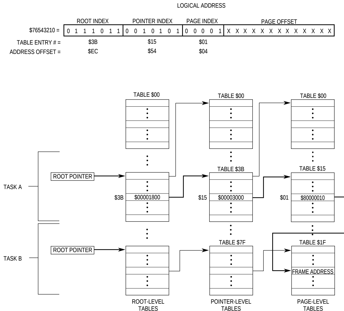
Figure 3-14. Translation Table Using Indirect Descriptors
