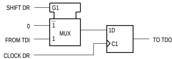
Figure C-5. Bypass Register
