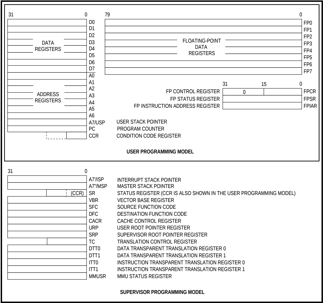
Figure 1-2. Programming Model
