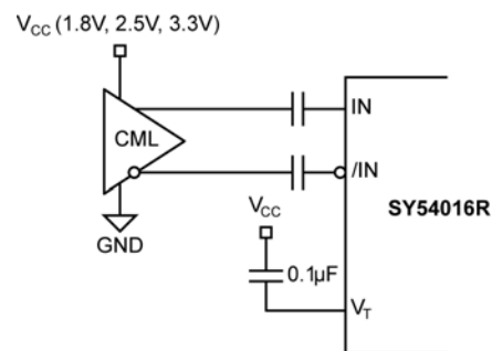
Figure 4c. CML Interface (AC-Coupled)
