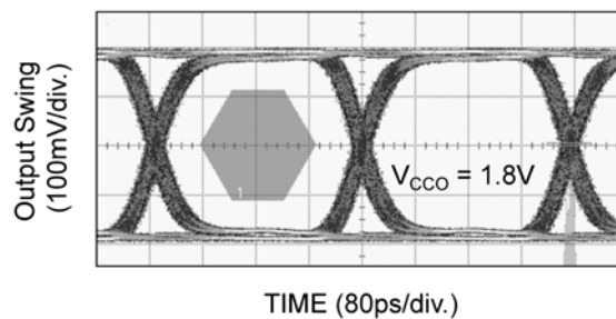
3.2Gbps Data
