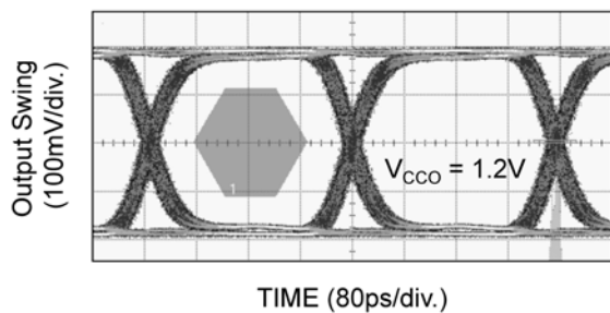
3.2Gbps Data
