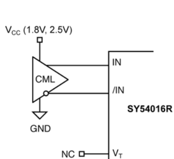
Figure 4a. CML Interface (DC-Coupled, 1.8V, 2.5V)
