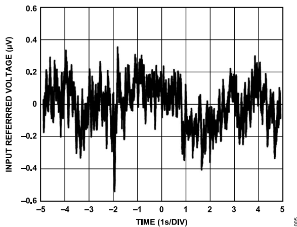
Figure 6. 0.1 Hz to 10 Hz Noise Peak to Peak, I_{CQ1} = 100 \mu A and I_{BZ1} = 5 \text{ mA}
