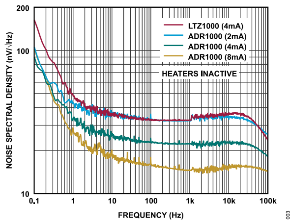
Figure 3. Noise Spectral Density vs. Frequency, LTZ1000 and ADR1000 with Various I_{BZ1} , I_{CQ1} = 100 \mu A (Heater Inactive)
