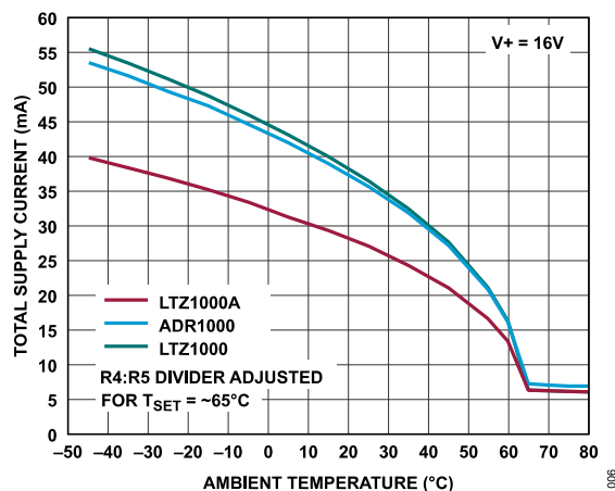
Figure 7. Total Supply Current vs. Ambient Temperature, ADR1000, LTZ1000, and LTZ1000A, Circuit of Figure 9 with R4:R5 Dividers Adjusted for T_{SET} \sim 65^\circ C
