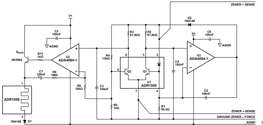
Figure 9. Typical Connection Diagram
