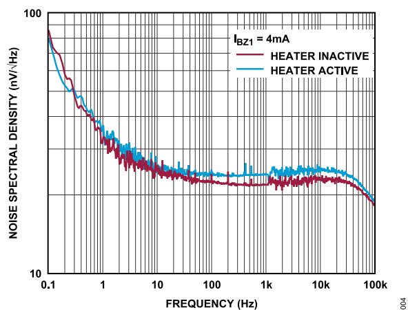
Figure 4. Noise Spectral Density vs. Frequency, Heater Active vs. Inactive, I_{BZ1} = 4 \text{ mA} , I_{CQ1} = 100 \mu A
