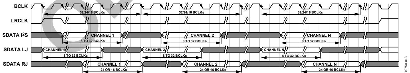
Figure 28. TDM Modes with Pulse Mode LRCLK
