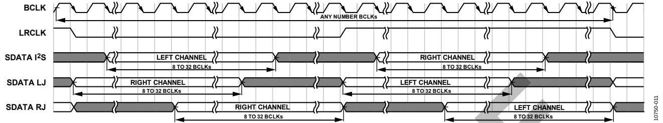
Figure 26. Stereo Modes: I 2 S, Left Justified, and Right Justified
