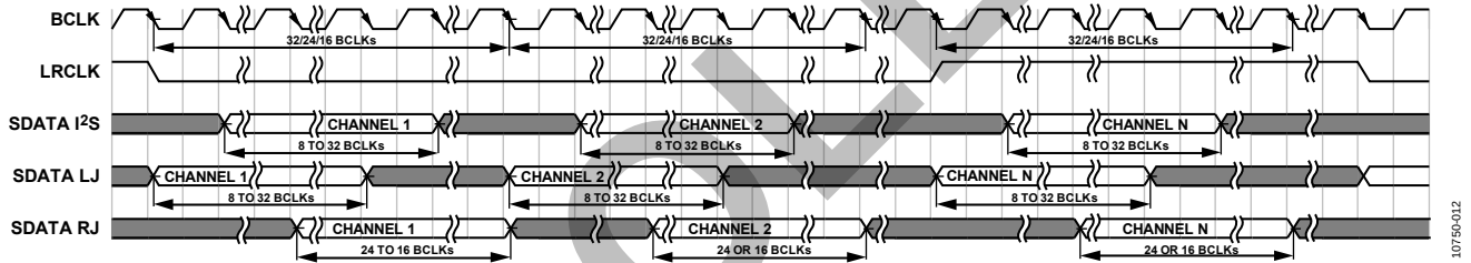
Figure 27. TDM Modes with 50% Duty Cycle LRCLK
