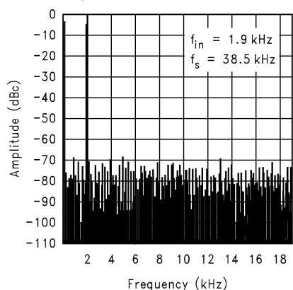
Spectral Response with 1.9 kHz Sine Wave Input, f_{CLK} = 500 kHz
