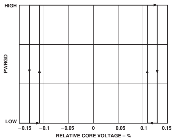
TPC 4. Power Good vs. Relative Core Voltage Variation
