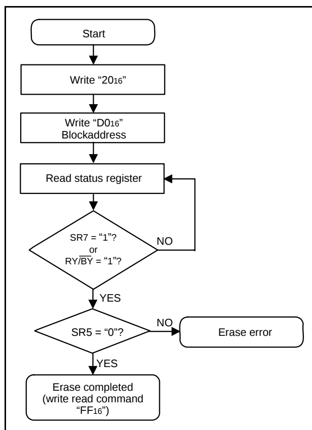
Fig. 87 Erase flowchart
