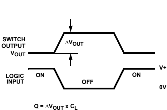
FIGURE 2A. MEASUREMENT POINTS
