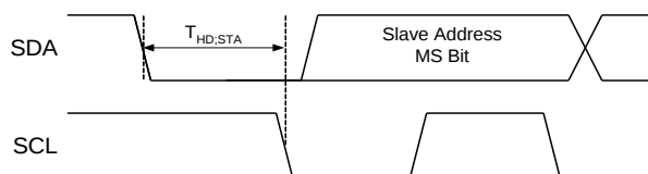
Figure 24. Start Bit
