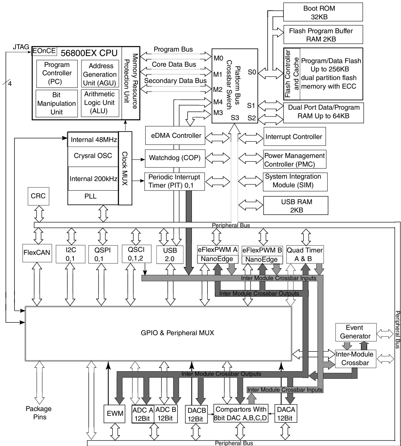
Figure 2. System diagram
