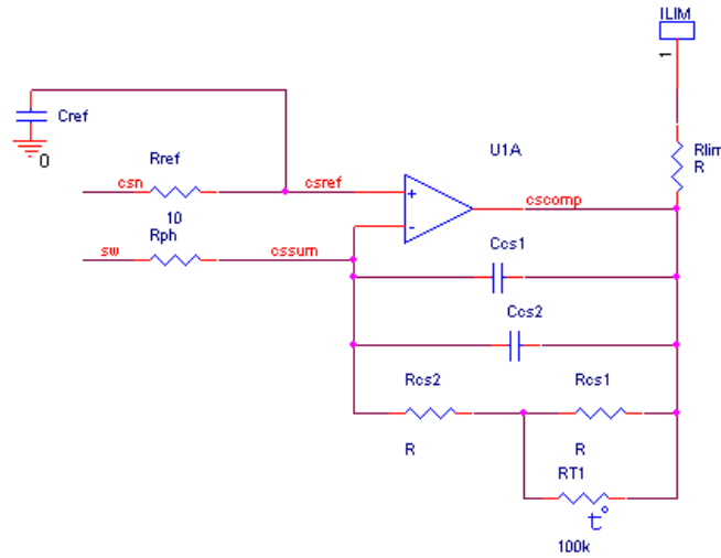
Figure 14. Current Limit
