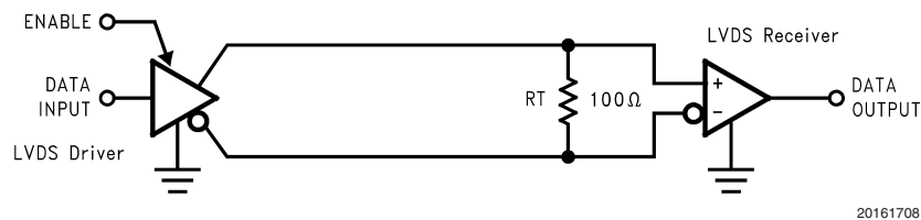
FIGURE 10. Point-to-Point Application
