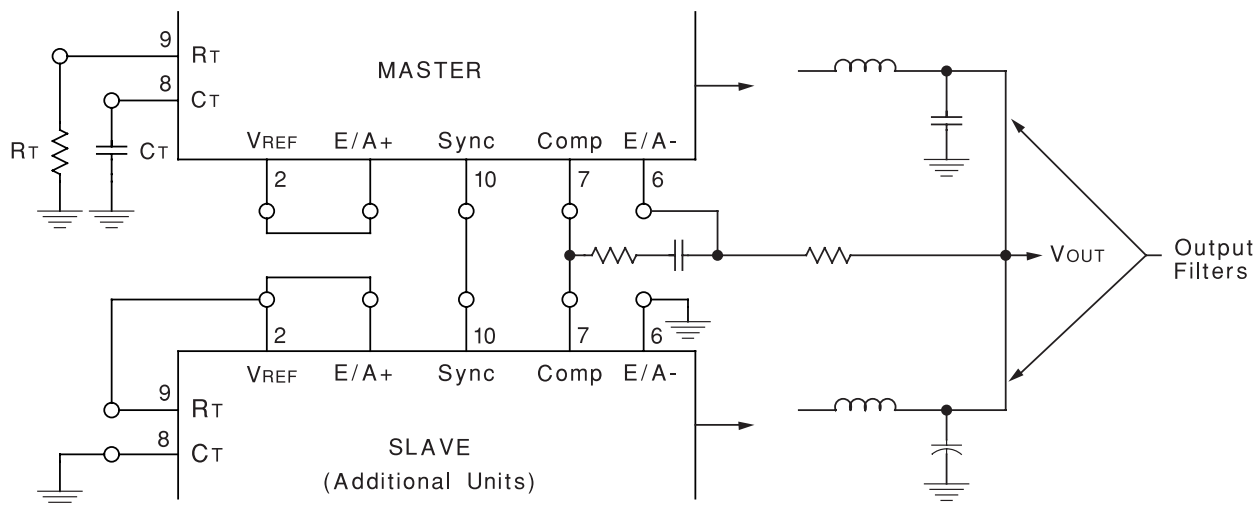
Figure 13. Parallel Operation
