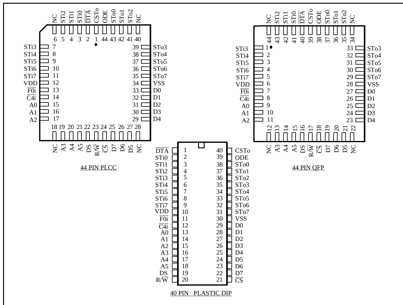
Figure 2 - Pin Connections
