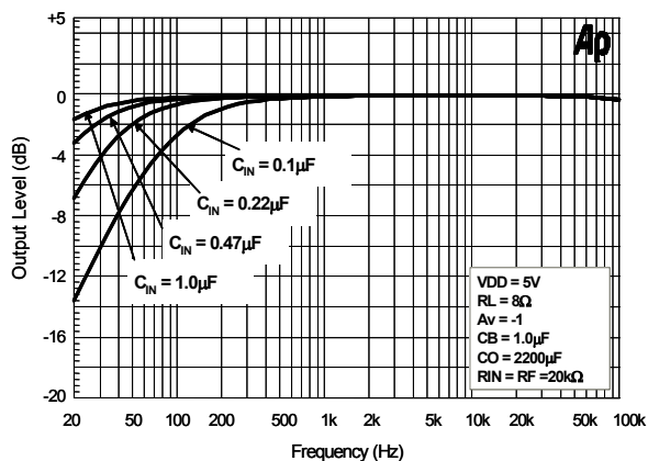
Figure 18. Output Level vs. Frequency
