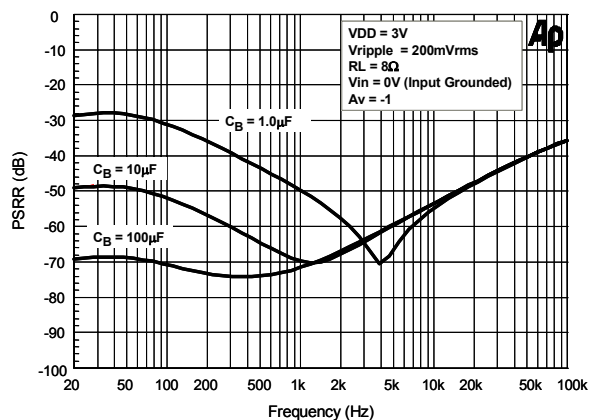
Figure 14. Power Supply Rejection Ratio
