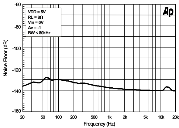
Figure 21. Noise Floor
