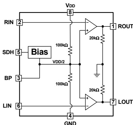
FAN7005M(8SOP)
