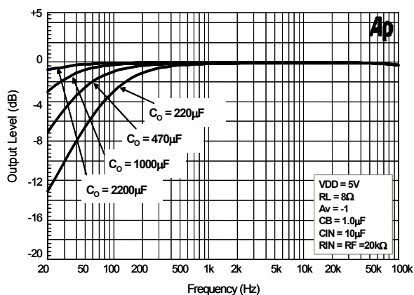
Figure 16. Output Level vs. Frequency
