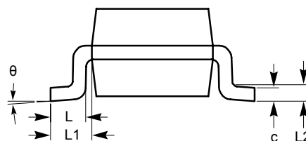
END VIEW
