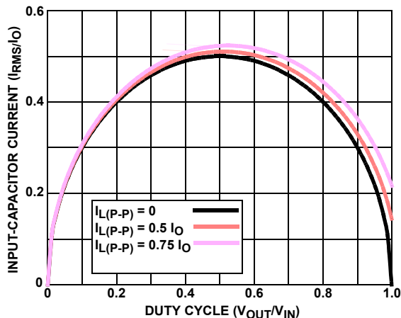
FIGURE 40. NORMALIZED INPUT-CAPACITOR RMS CURRENT vs DUTY CYCLE FOR SINGLE-PHASE CONVERTER
