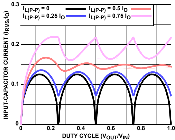
FIGURE 39. NORMALIZED INPUT-CAPACITOR RMS CURRENT vs DUTY CYCLE FOR 4-PHASE CONVERTER
