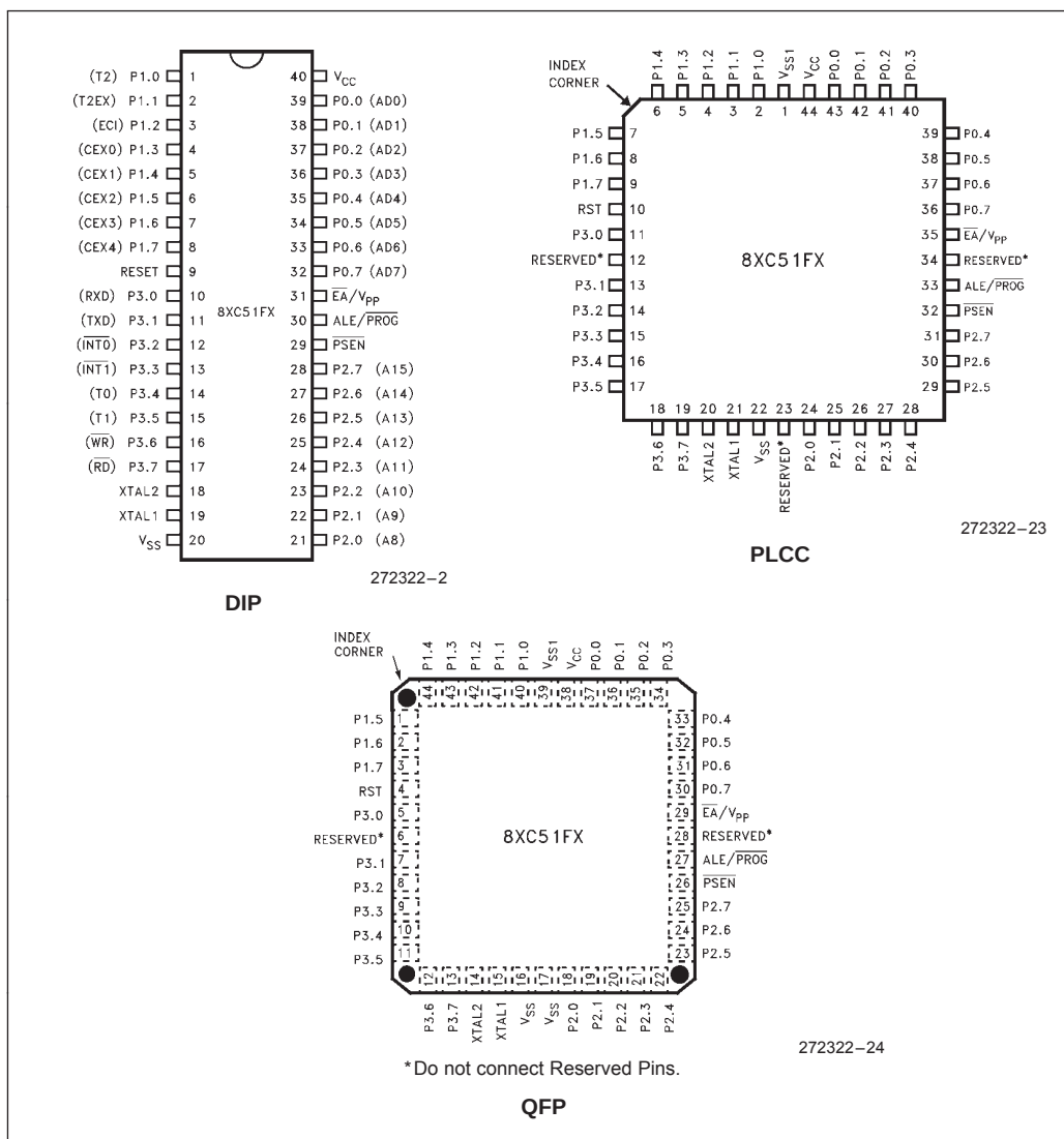
Figure 2. Pin Connections
