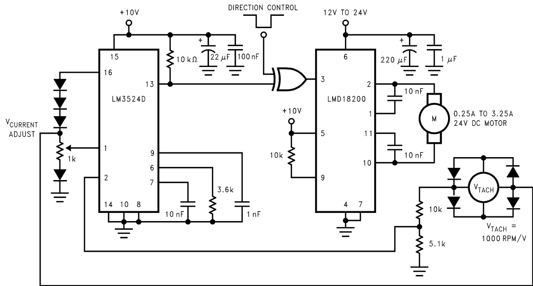
Figure 20. Regulate Velocity with Tachometer Feedback
