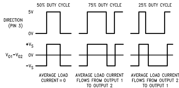
Figure 11. Locked Anti-Phase PWM Control
