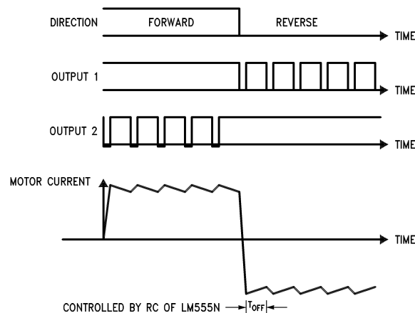
Figure 17. Switching Waveforms
