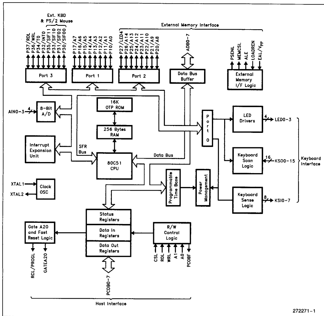
Figure 1. Block Diagram
