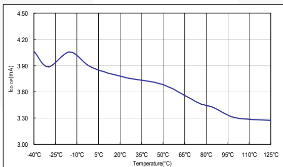
Figure 9. Operating Current
