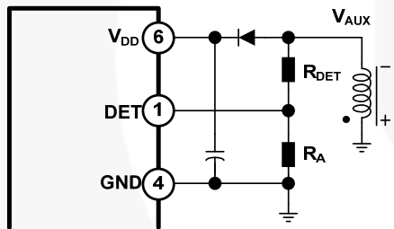
Figure 17. Valley Detect Section
