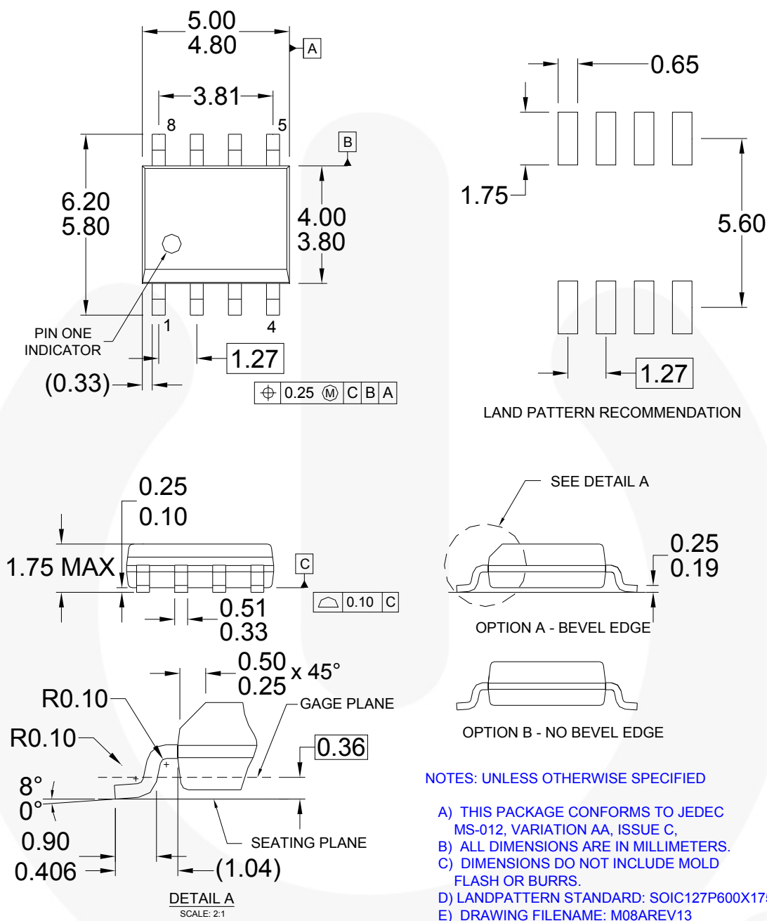
Figure 24. 8-Pin Small Outline Package (SOP)
