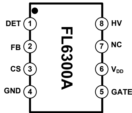
Figure 4. Pin Assignments
