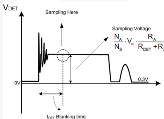
Figure 23. Voltage Sampled After 4 \mu s Blanking Time After Switch-Off Sequence
