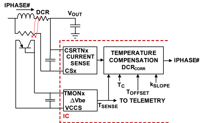
FIGURE 14. BLOCK DIAGRAM OF TEMPERATURE COMPENSATION
