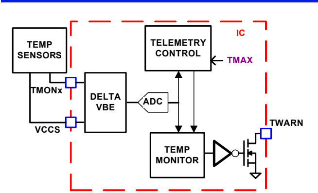
FIGURE 23. BLOCK DIAGRAM OF THERMAL MONITORING FUNCTION
