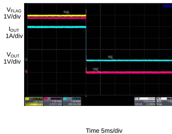
Figure 19. FLAG Response during Over Temperature ( T_A=125^{\circ}C )
