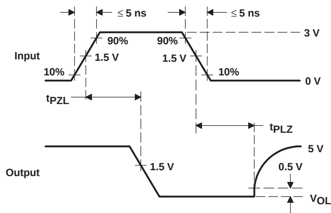
VOLTAGE WAVEFORMS
