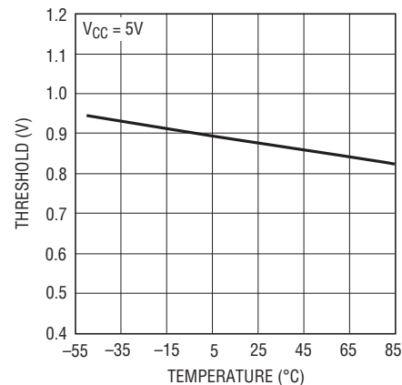
SUSP/HPWR Pin Rising Thresholds vs Temperature
