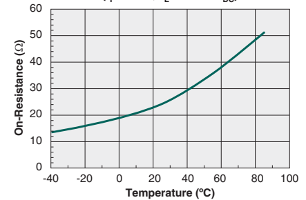
Typical On-Resistance vs. Temperature ( I_F=5\text{mA} , I_L=100\text{mA}_{\text{DC}} )
