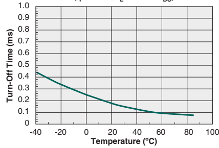
Typical Turn-Off vs. Temperature ( I_F=5\text{mA} , I_L=100\text{mA}_{\text{DC}} )
