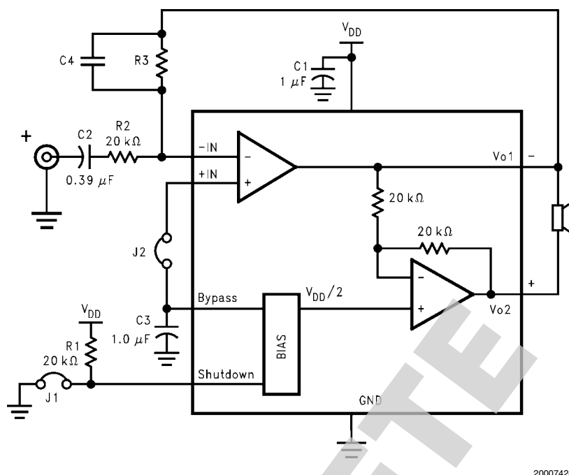
FIGURE 2. Higher Gain Audio Amplifier
