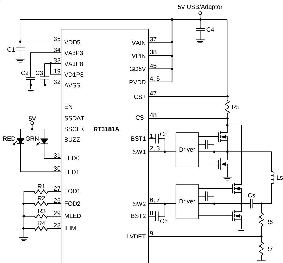
Figure 2. WPC LP A11 High Performance Transmitter Application Circuit
