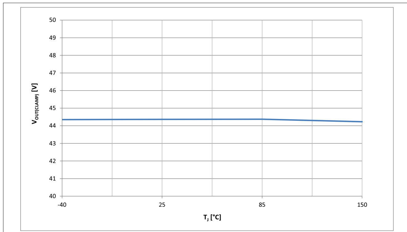
Figure 38 Typical V_{OUT(CLAMP)} vs. T_J @ I_L = 10 mA
