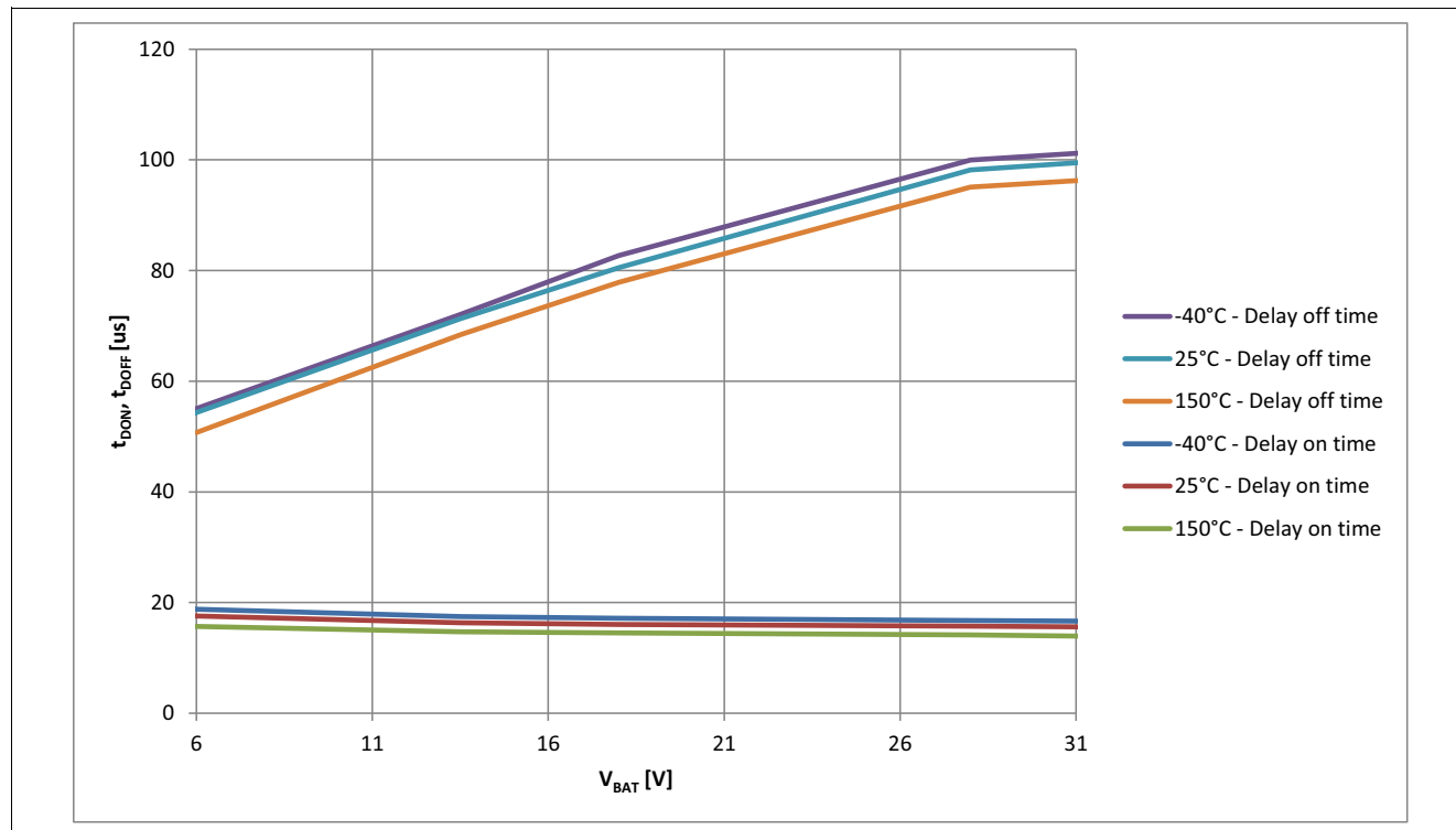
Figure 30 Typical t_{DON} , t_{DOFF} vs V_{BAT} @ V_{IN} = 5 V, T_J = -40 \dots 150^\circ\text{C}
