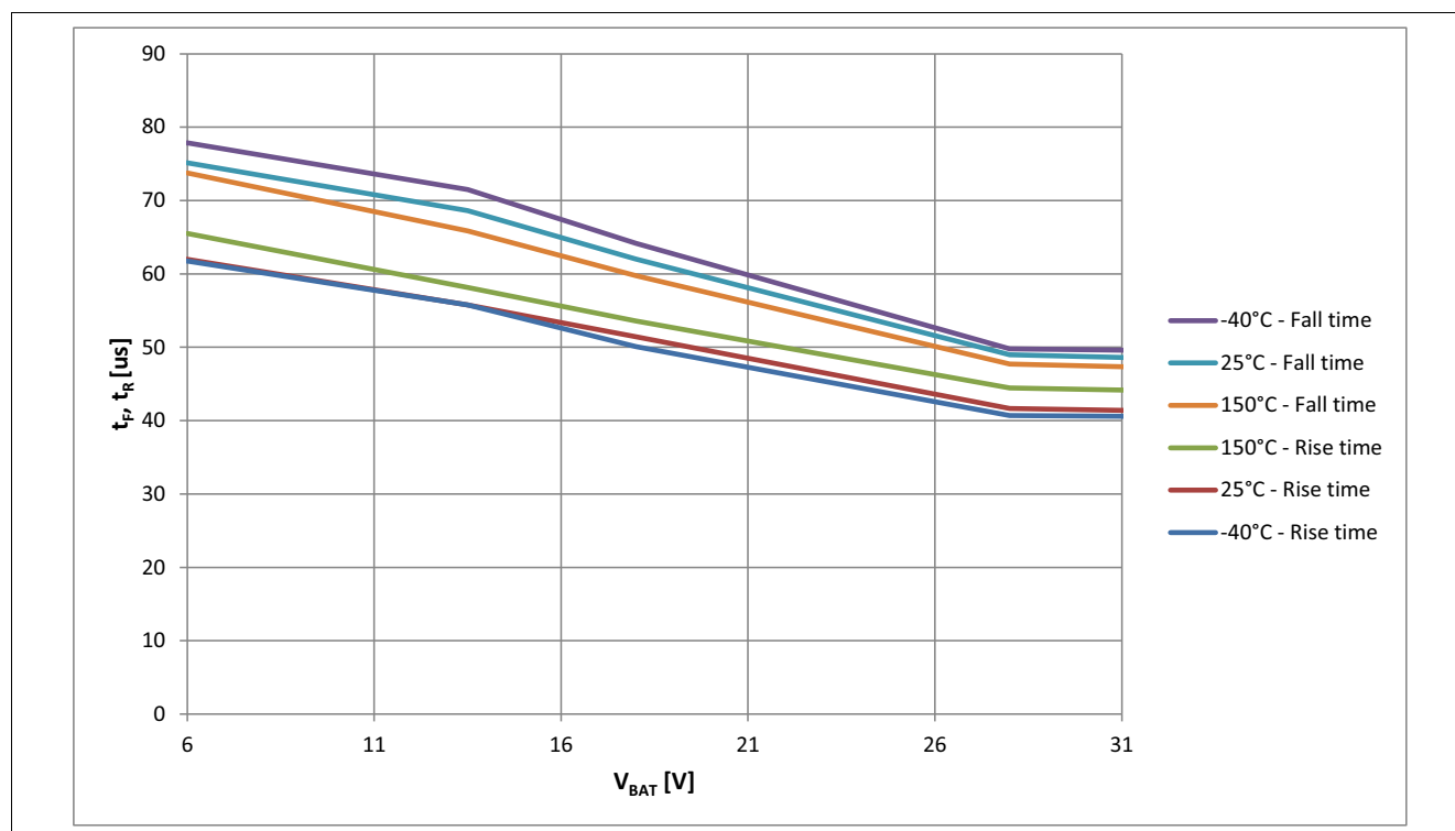
Figure 29 Typical t_F , t_R vs V_{BAT} @ V_{IN} = 5 V, T_J = -40 \dots 150^\circ\text{C}
