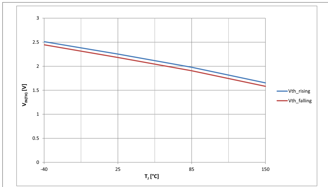
Figure 40 Typical V_{IN(TH)} vs. T_J @ I_L = 1 mA
