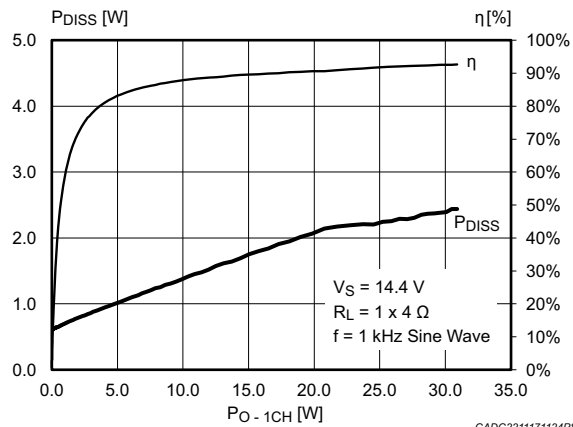
Figure 4. Efficiency and power dissipation ( V_S = 14.4\text{ V} , R_L = 1 \times 4\ \Omega , f = 1\text{ kHz} sine wave)
