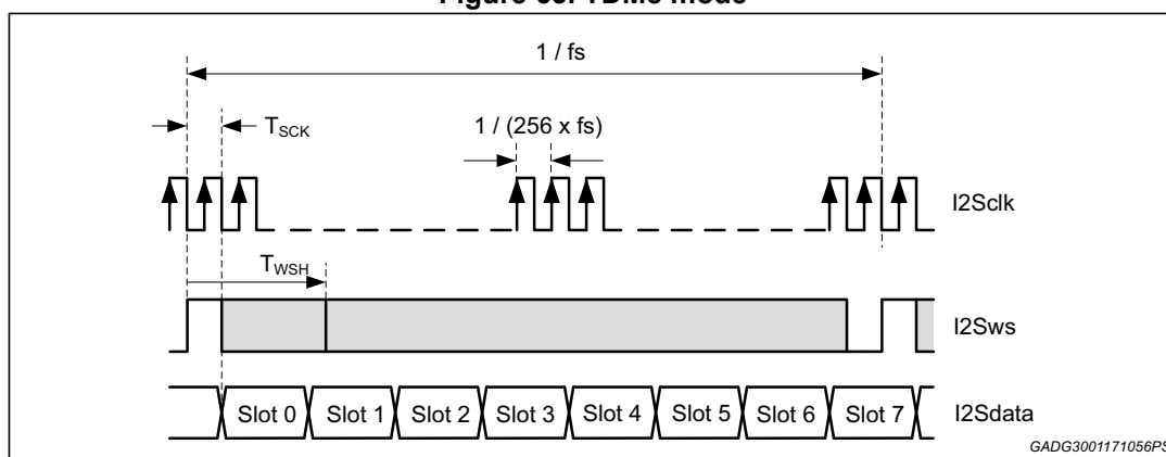
Figure 65. TDM8 mode
