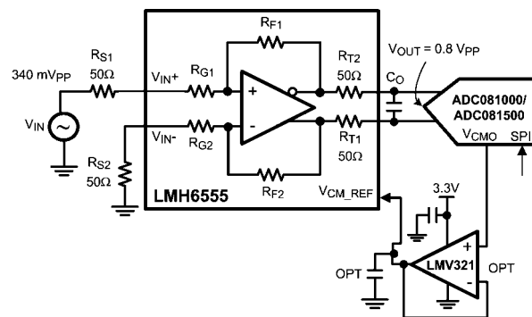
FIGURE 19. Increasing ±0.5 dB Gain Flatness using External Output Capacitance, C O
