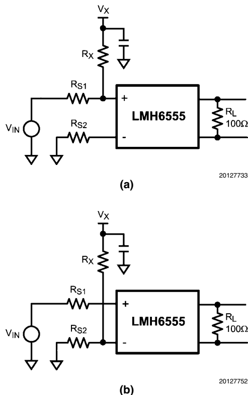
FIGURE 9. Differential Output Shift Circuits
