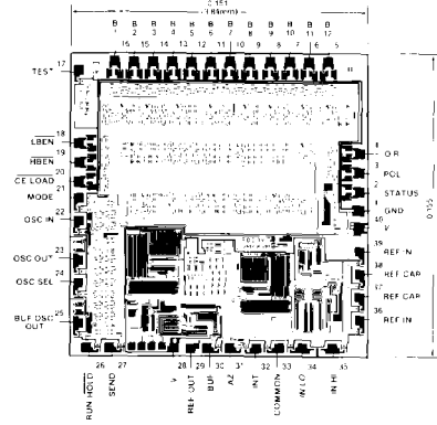
Chip Topography
