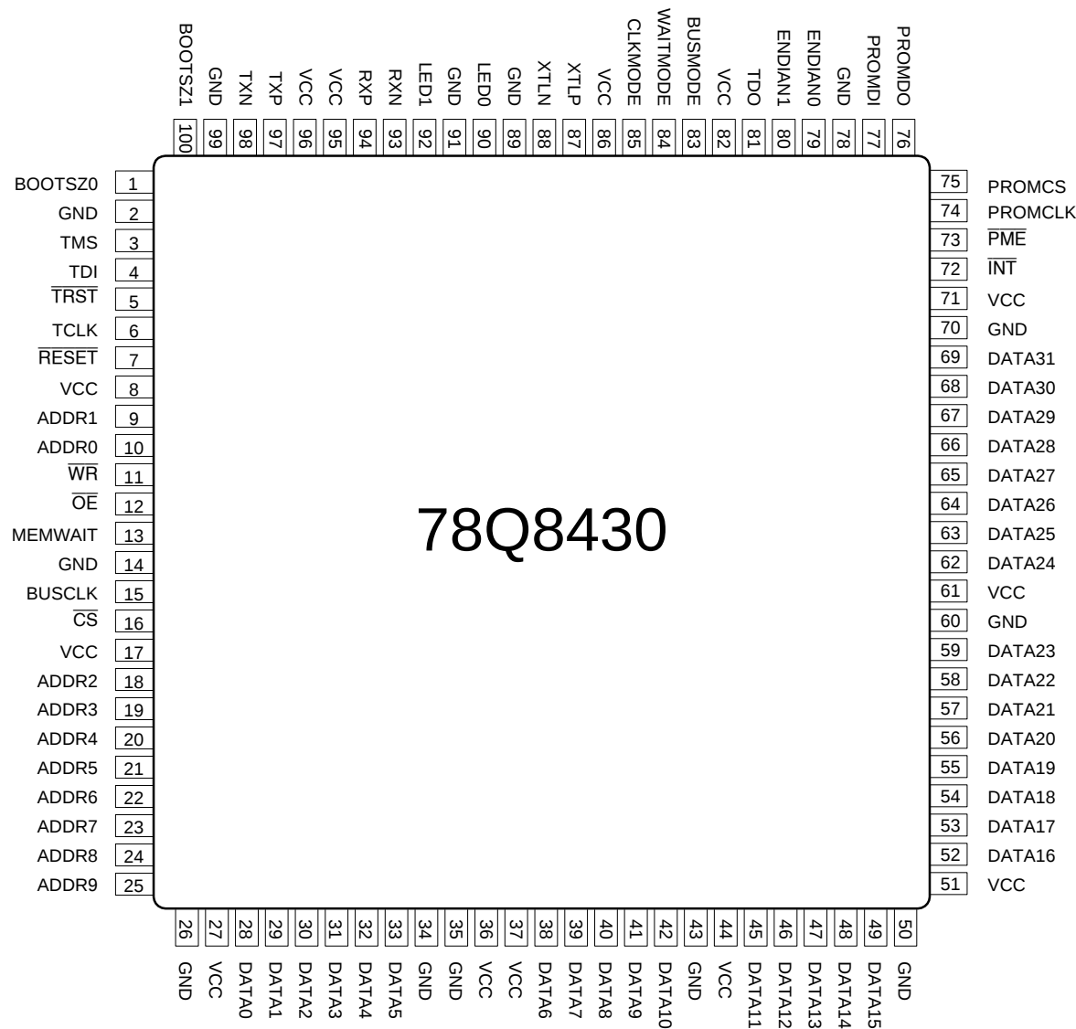
Figure 7: Pinout
