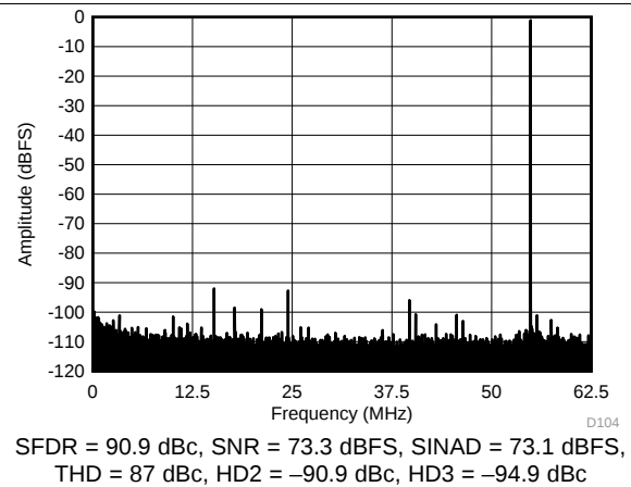
Figure 97. FFT for 70-MHz Input Signal (Dither Off)
