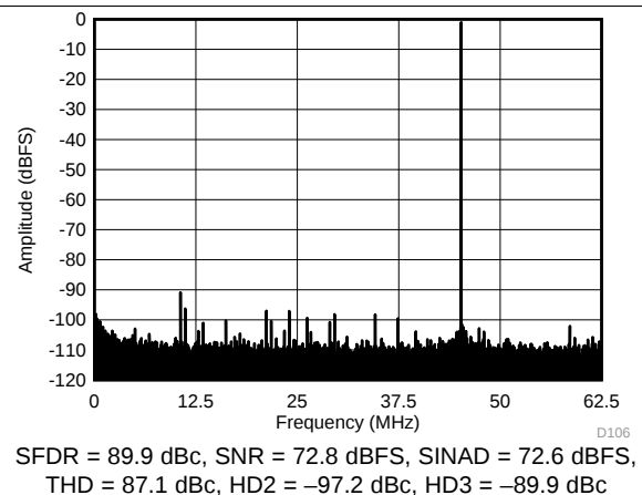
Figure 99. FFT for 170-MHz Input Signal (Dither Off)
