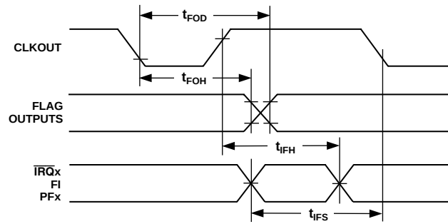
Figure 22. Interrupts and Flags
