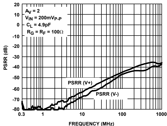
FIGURE 9. PSRR CHANNELS
