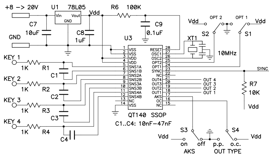
Figure 1-6 Basic Circuit (QT140, SSOP Package)
