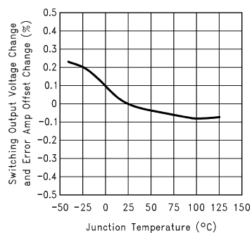
Normalized Error Amplifier Voltage vs Junction Temperature
