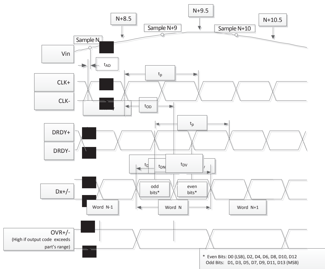
Figure 1. Output Timing
