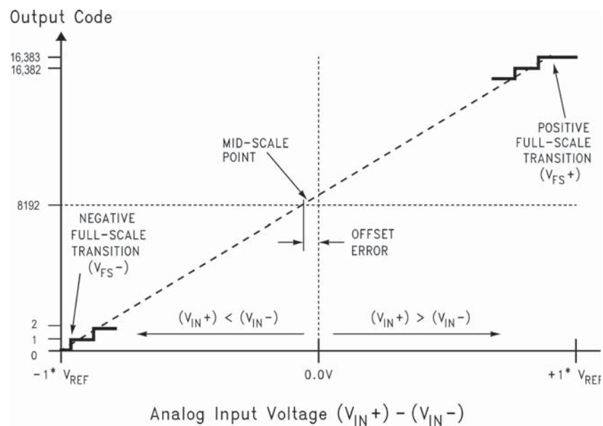
Figure 2. Transfer Characteristic (Offset Binary Format)
