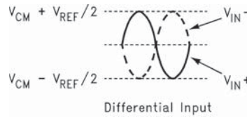
Figure 20. Expected Input Signal Range
