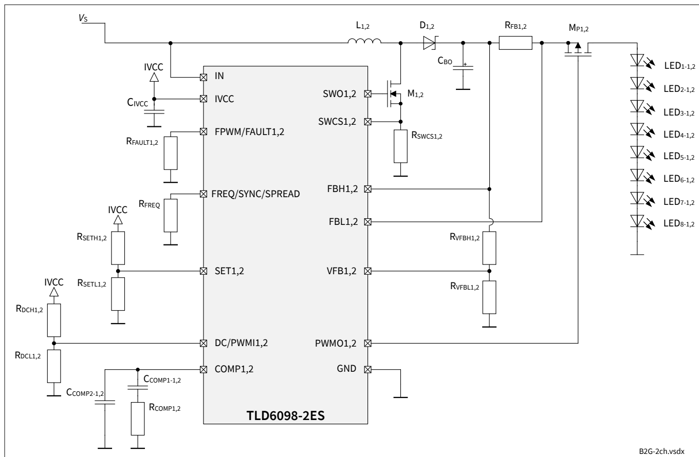
Figure 1 Application diagram
